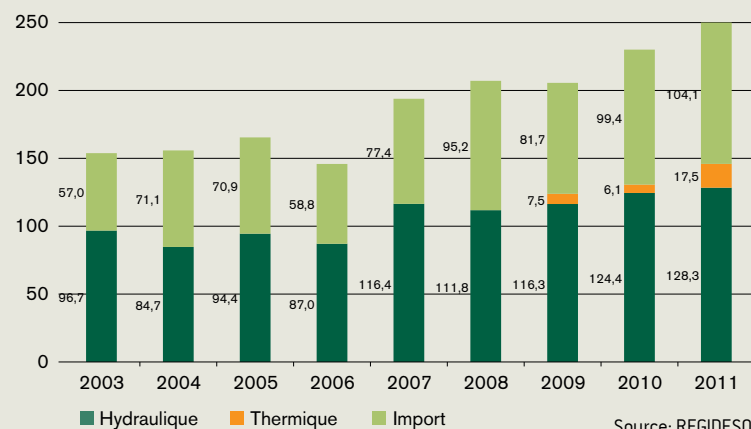
Figure 6 Sources de production de la REGIDESO (2003-2011)
